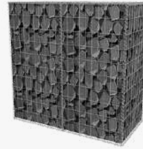
Gabion plein concassé calcaire noir, dim.L100xI100xH50cm, dim. fil 5.8 mm
